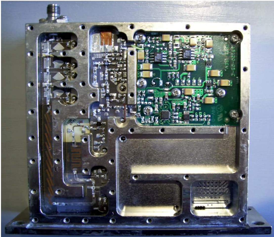
RF side of the synthesiser showing the hairpin and stripline filters at the bottom left.
